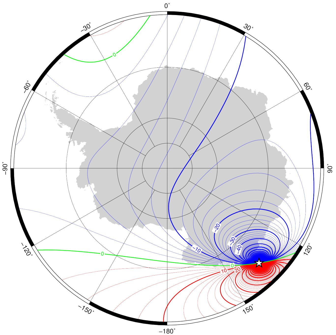
Annual rate of change of declination in region of south pole for 2020.0 to 2025.0 from the World Magnetic Model (WMM2020). Red – easterly change, blue – westerly change, green – zero change. Contour interval is 2'/year, white star is location of a magnetic pole and projection is Polar Stereographic. Credit: British Geological Survey (UK Research and Innovation).
