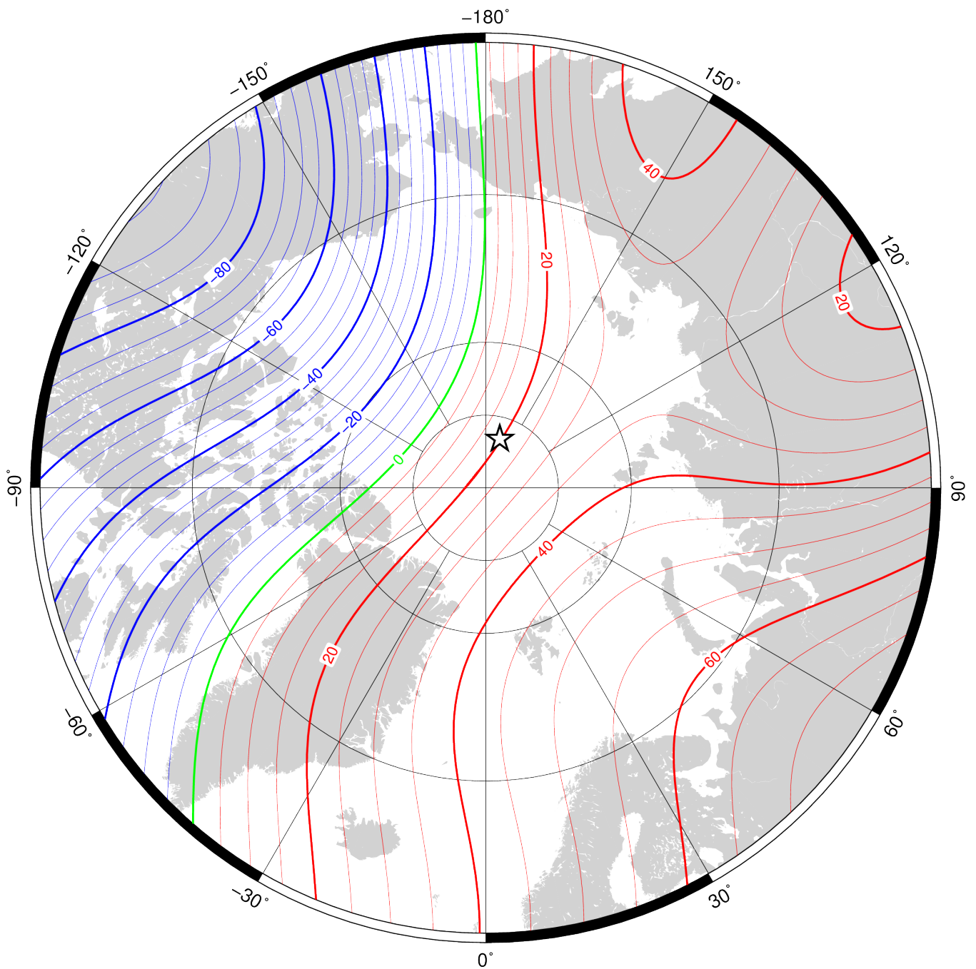
Annual rate of change of total intensity in region of north pole for 2020.0 to 2025.0 from the World Magnetic Model (WMM2020). Red – positive change, blue – negative change, green – zero change. Contour interval is 5 nT/year, white star is location of a magnetic pole and projection is Polar Stereographic. Credit: British Geological Survey (UK Research and Innovation).
