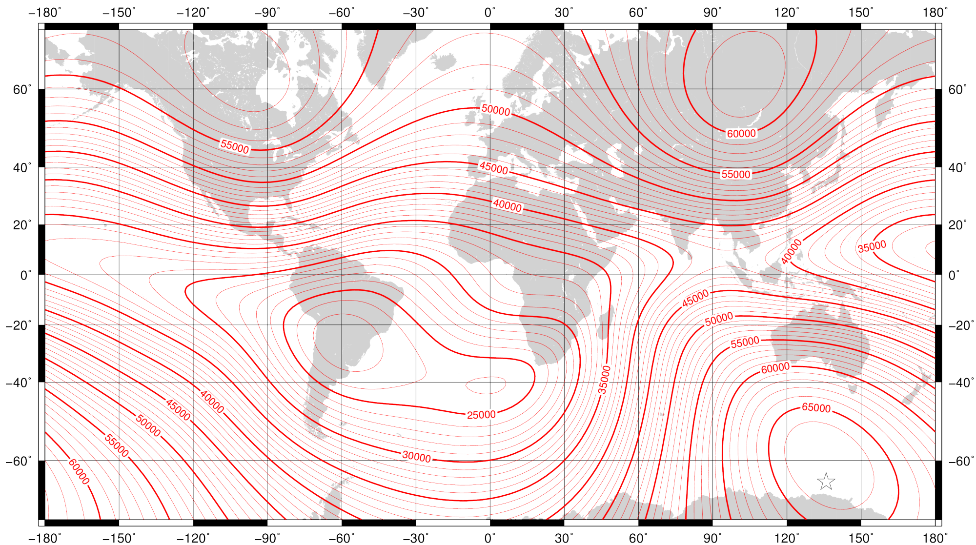
Total intensity ( F ) at 2020.0 from the World Magnetic Model (WMM2020). Contour interval is 1000 nT, white star is location of a magnetic pole and projection is Mercator. This is an example of an isodynamic chart. Credit: British Geological Survey (UK Research and Innovation).
