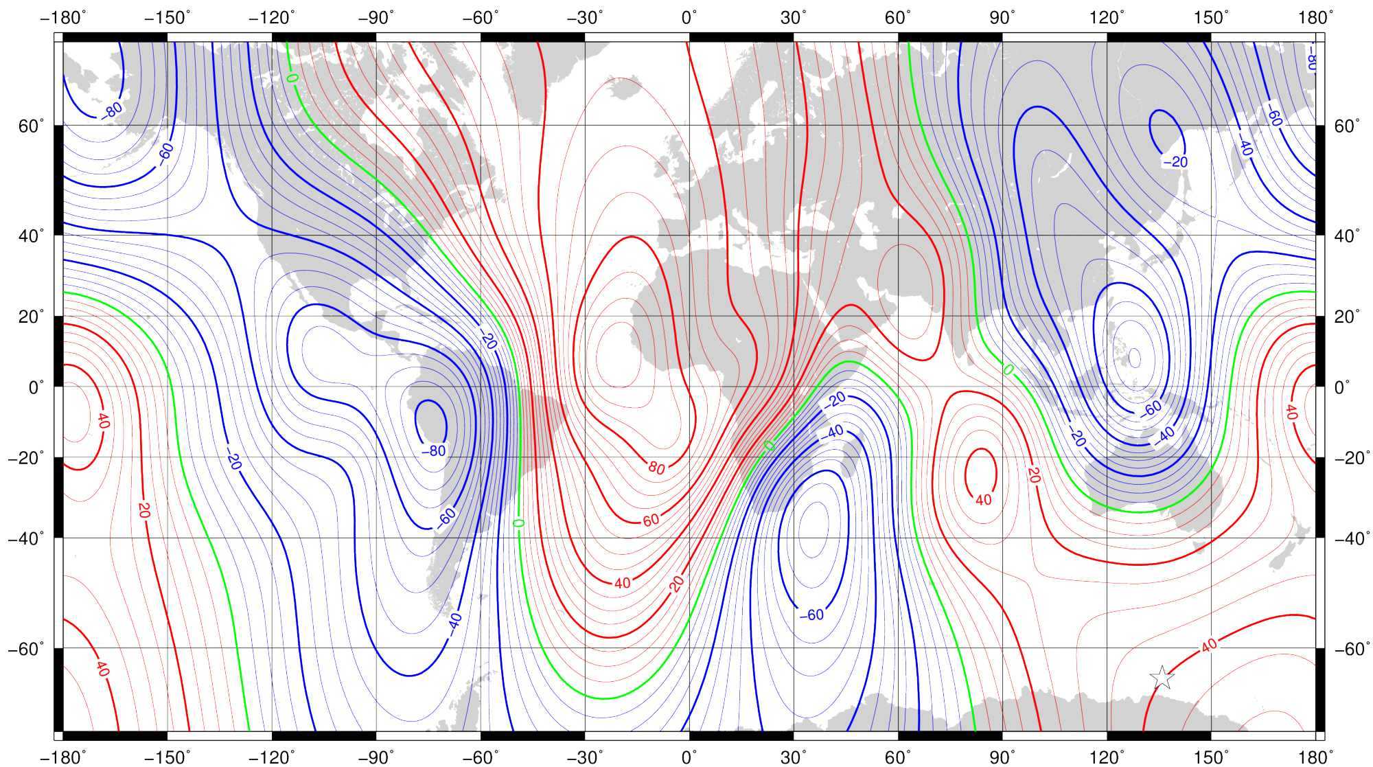
Annual rate of change of east component for 2020.0 to 2025.0 from the World Magnetic Model (WMM2020). Red – positive change, blue – negative change, green – zero change. Contour interval is 5 nT/year, white star is location of a magnetic pole and projection is Mercator. This is an example of an isoporic chart. Credit: British Geological Survey (UK Research and Innovation).
